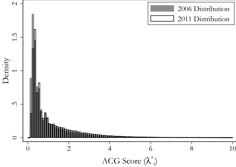
Figure 2: Distribution of \lambda_t^* in 2006 and 2011
