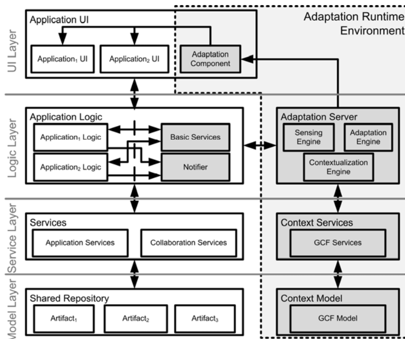
Figure 28 Conceptual Architecture
